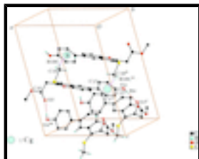
Fig. 2. O—H...O and C—H... \pi interactions (dotted lines) in the title compound. Cg denotes the ring centroid. [Symmetry codes: (i) -x + 1, y + 1, -z + 3/2 ; (ii) -x + 1, -y + 1, -z + 1 ; (iii) -x + 1, y - 1/2, -z + 3/2 .]
